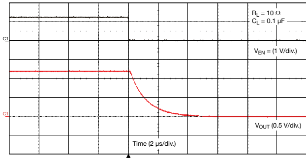
Fig. 22 - Turn-Off Time ( V_{IN} = 1.2\text{ V} )
