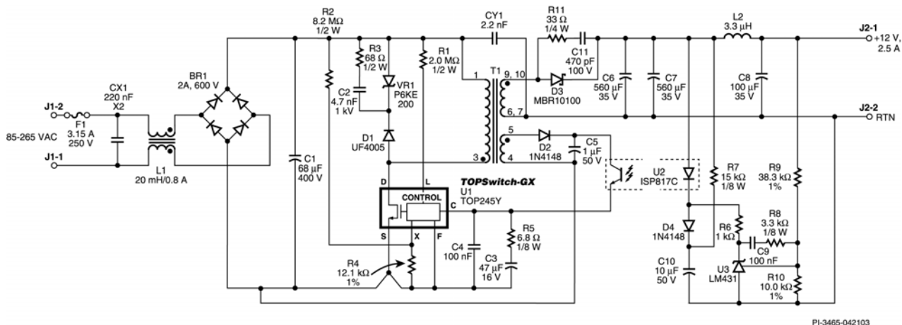
Figure 2 – EP-34 Schematic.
