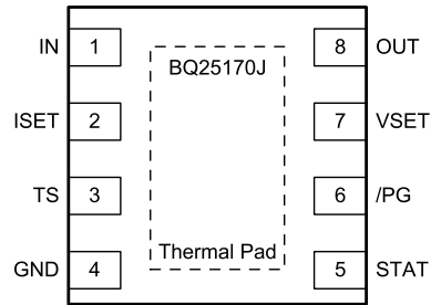
Figure 5-1. WSON Package 8-Pin Top View
