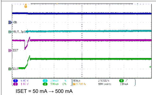
Figure 8-12. ISET Change Response
