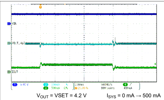
Figure 8-9. OUT Transient Response
