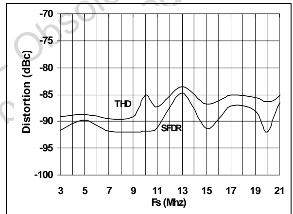
Fig. 14: Distortion vs. F_s at F_{in}=5\text{MHz} , using TS4041 I_{cca} optimised; V_{REFP}=1.225\text{V} ; V_{REFM}=\text{GND} ; INCM=0.65\text{V}
