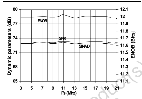
Fig. 14: Distortion vs. F_s at F_{in}=5\text{MHz} , using TS4041 I_{cca} optimised; V_{REFP}=1.225\text{V} ; V_{REFM}=\text{GND} ; INCM=0.65\text{V}
