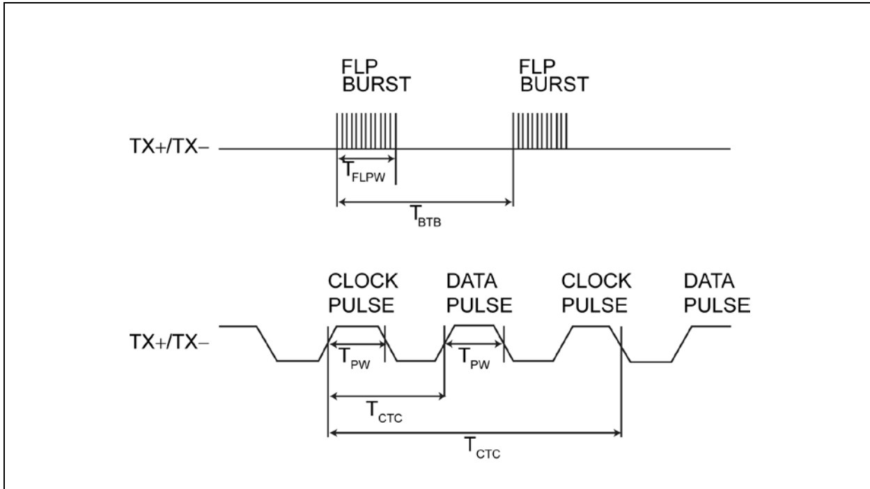
FIGURE 7-2: AUTO-NEGOTIATION TIMING
