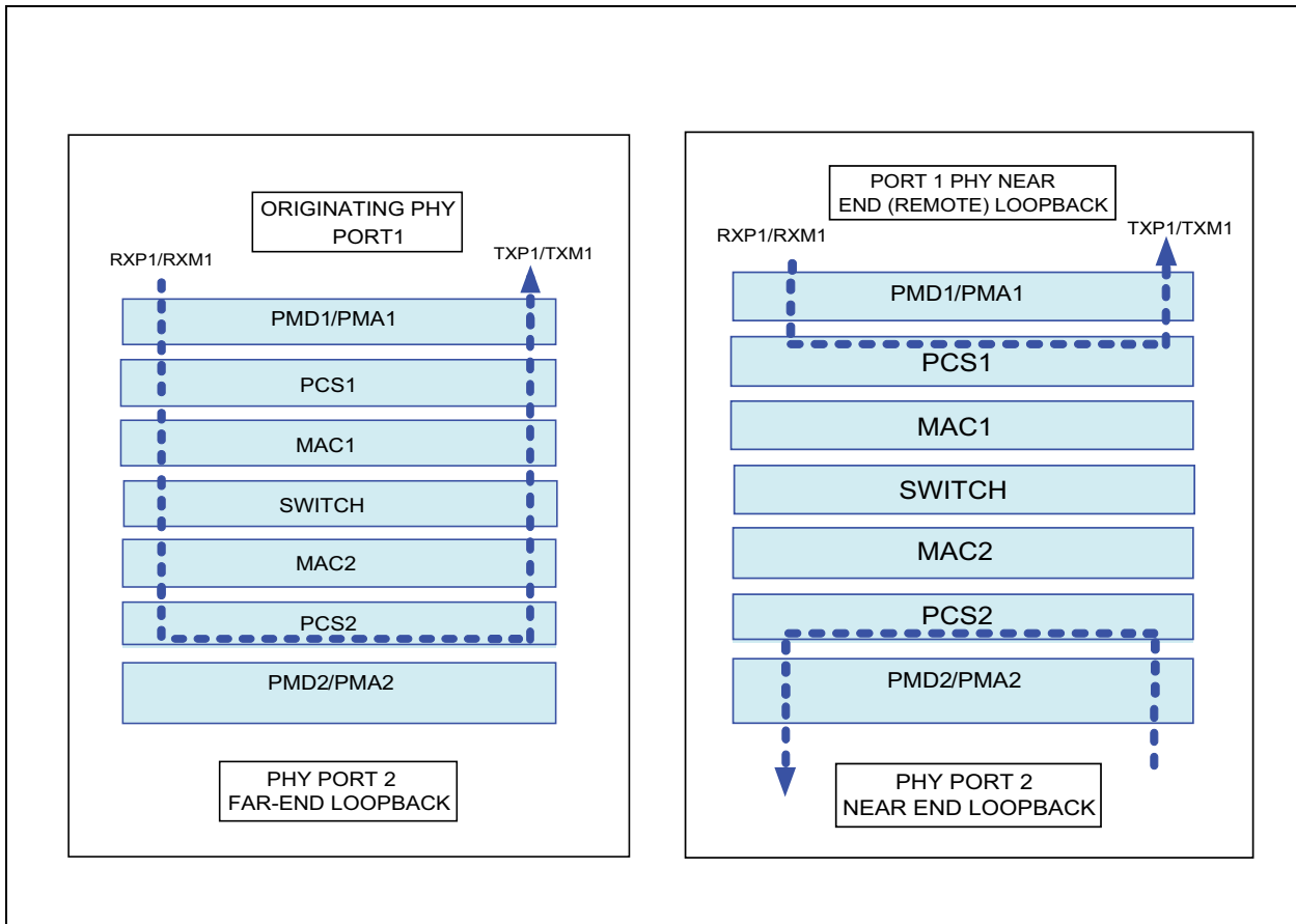
FIGURE 3-4: NEAR-END AND FAR-END LOOPBACK
