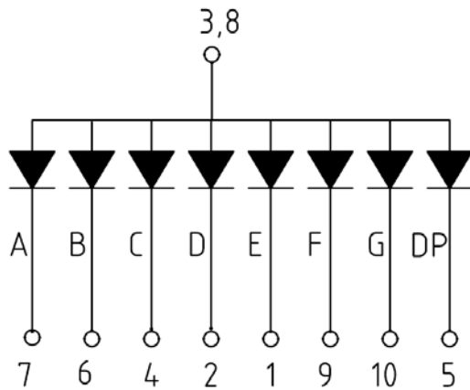
Common Anode
