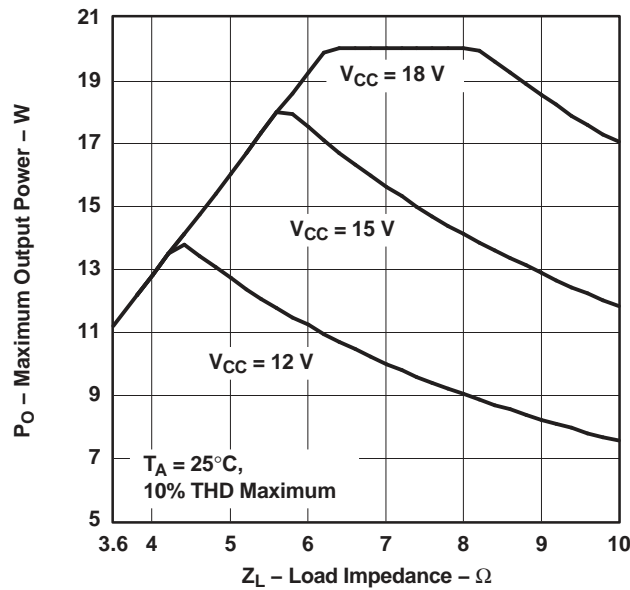
Figure 33. Output Power
