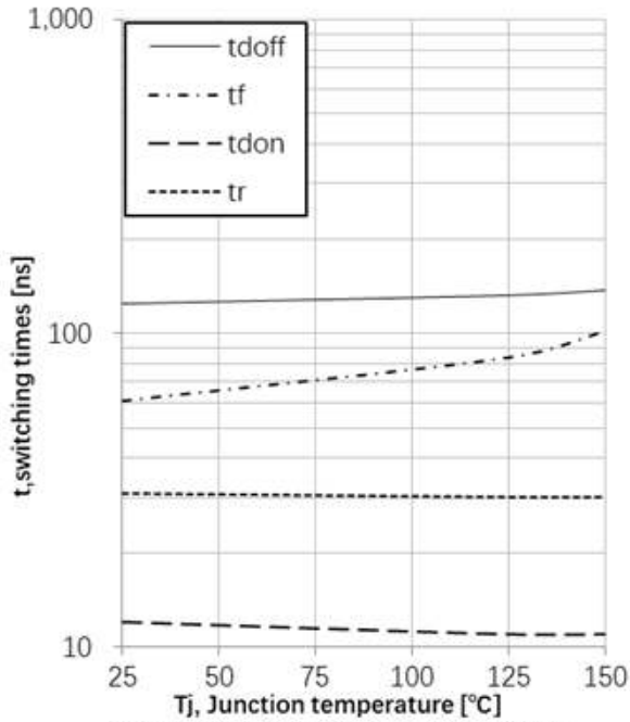
Fig9. Typical switching times as a function of junction temperature (inductive load, I_c=40A, V_{ce}=400V, V_{ge}=0/15V, R_g=10\Omega )
