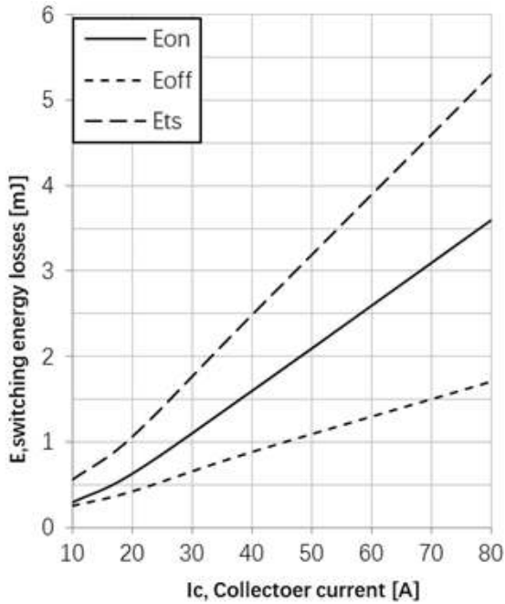
Fig11. Typical switching energy losses as a function of collect current (inductive load, T_{vj}=150^\circ C, V_{ce}=400V, V_{ge}=0/15V, R_g=10\Omega )
