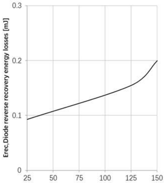
Tj, Junction temperature [°C] Fig21. Typical diode reverse recovery energy losses as a fuction of Junction temperature (inductive load, If=40A, Vrr=400V)
