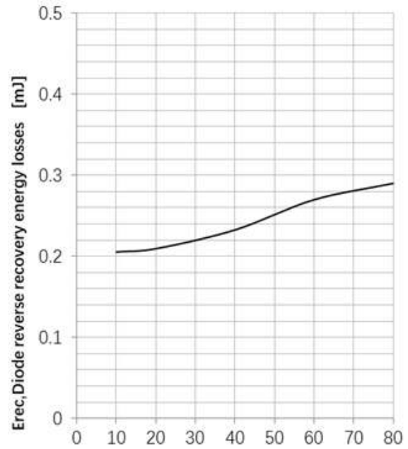
If, Collectoer current [A] Fig22. Typical diode reverse recovery energy losses as a fuction of collect current (inductive load, Tvj=150°C, Vrr=400V)
