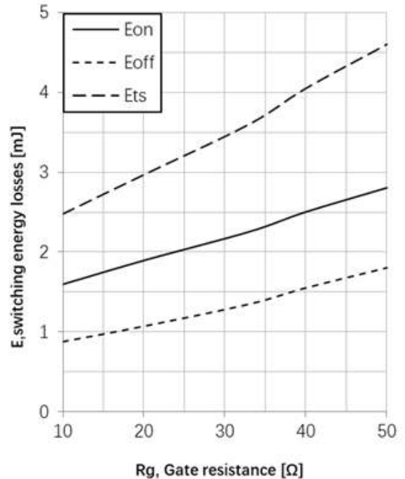
Fig12. Typical switching energy losses as a function of gate resistance (inductive load, T_{vj}=150^\circ C, V_{ce}=400V, V_{ge}=0/15V, I_c=40A )
