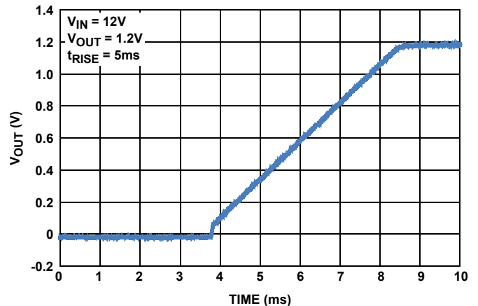
FIGURE 14. SOFT-START RAMP-UP
