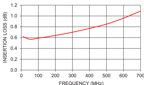
TC2-72T-5+ INSERTION LOSS
