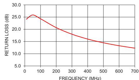
TC2-72T-5+ INPUT RETURN LOSS
