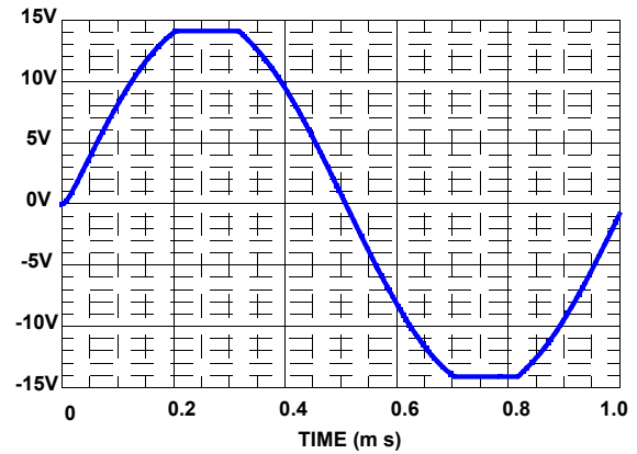
FIGURE 61. SIMULATED OUTPUT VOLTAGE SWING \pm 15V
