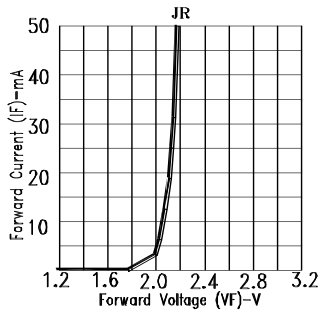
Fig3. FORWARD CURRENT VSE FORWARD VOLTAGE
