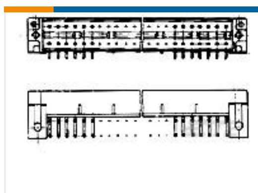
TE Part #172457-2 POST HDR ASSY 40P MULTI TAP
