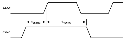
Figure 8. SYNC Input Timing Requirements
