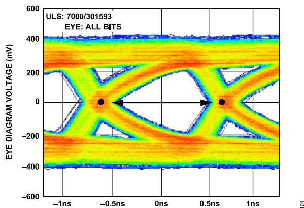
Figure 73. Data Eye for LVDS Outputs in ANSI-644 Mode with Trace Lengths Greater than 24 Inches on Standard FR-4 Material, External 100 Ω Far-End Termination Only
