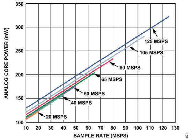
Figure 68. Analog Core Power vs. f_{SAMPLE} for f_{IN} = 10.3 MHz
