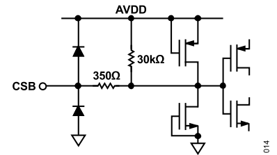
Figure 52. Equivalent CSB Input Circuit
