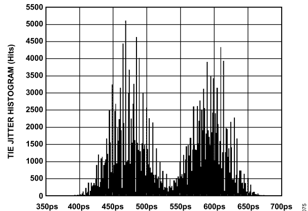
Figure 72. Time Interval Error (TIE) Jitter Histogram for LVDS Outputs in ANSI-644 Mode with Trace Lengths Less than 24 Inches on Standard FR-4 Material, External 100 Ω Far-End Termination Only
