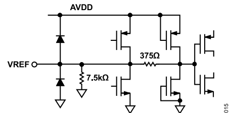
Figure 53. Equivalent VREF Circuit
