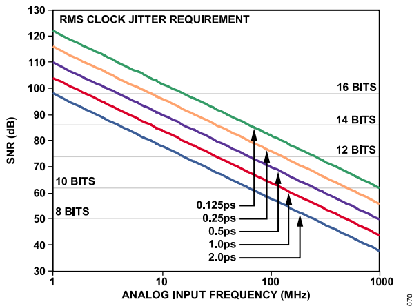
Figure 67. Ideal SNR vs. Input Frequency and Jitter
