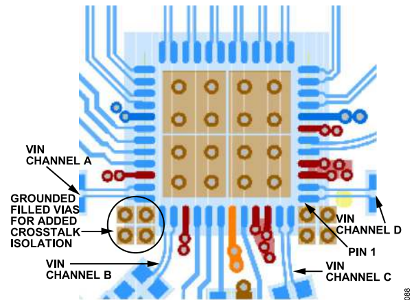
Figure 77. Layout Technique to Maximize Crosstalk Performance
