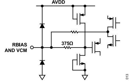
Figure 51. Equivalent RBIAS and VCM Circuit
