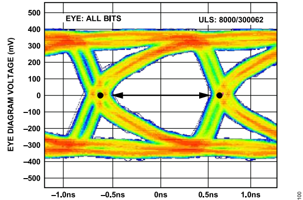
Figure 71. Data Eye for LVDS Outputs in ANSI-644 Mode with Trace Lengths Less than 24 Inches on Standard FR-4 Material, External 100 Ω Far-End Termination Only
