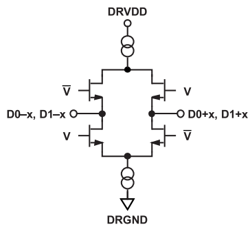
Figure 49. Equivalent Digital Output Circuit
