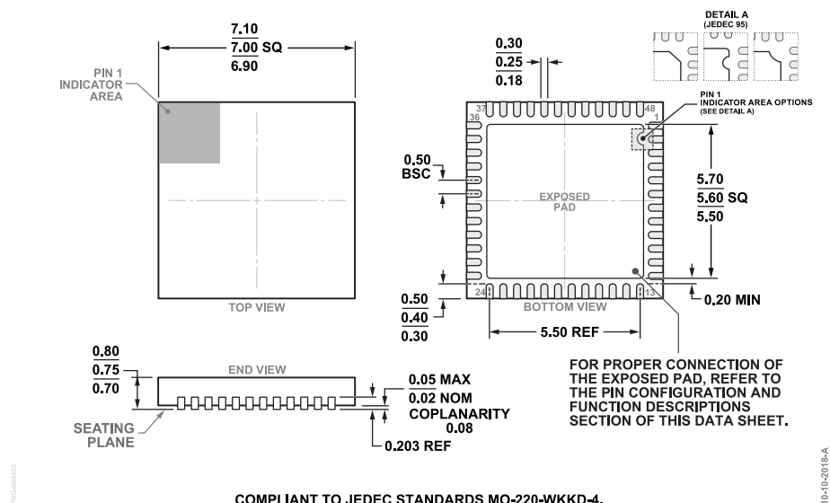
Figure 78. 48-Lead Lead Frame Chip Scale Package [LFCSP] 7 mm x 7 mm Body and 0.75 mm Package Height (CP-48-13) Dimensions shown in millimeters
