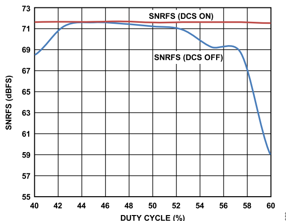
Figure 63. SNR vs. DCS On/Off
