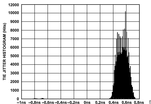
Figure 74. Time Interval Error (TIE) Jitter Histogram for LVDS Outputs in ANSI-644 Mode with Trace Lengths Greater than 24 Inches on Standard FR-4 Material, External 100 Ω Far-End Termination Only
