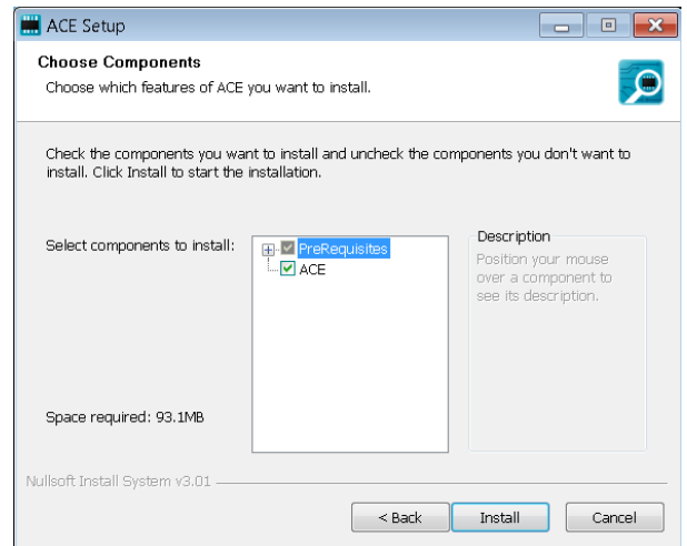
Figure 7. Choose Components
