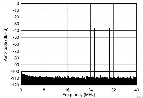
f_{IN1} = 185 \text{ MHz} , f_{IN2} = 190 \text{ MHz} , \text{IMD3} = 91 \text{ dBFS} , each tone at -36 \text{ dBFS}
