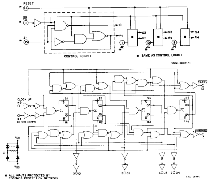
Fig. 1 — CD40192B logic diagram (BCD).
