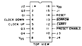
CD40192B, CD40193B TERMINAL ASSIGNMENT
