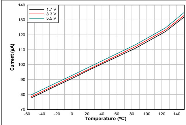
Figure 8-9. Temperature Conversion Current vs Temperature
