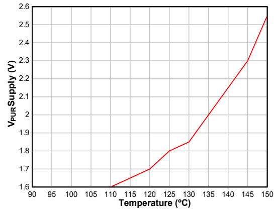
Figure 8-18. V_{PUR} Typical Standard Speed Mode Supply Voltage vs Temperature
