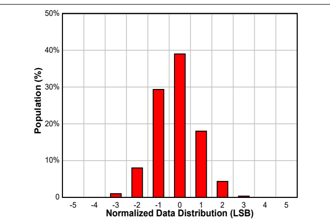
Figure 8-12. Data Distribution With 5.5-ms Conversion Time and Averaging On in 16-Bit Format
