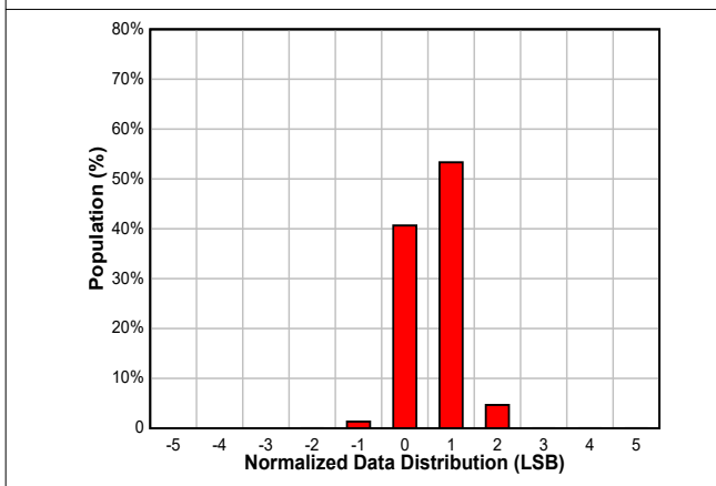
Figure 8-13. Data Distribution With 3-ms Conversion Time and Averaging On in 16-Bit Format
