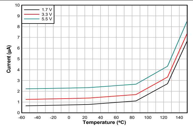
Figure 8-10. Shutdown Current vs Temperature
