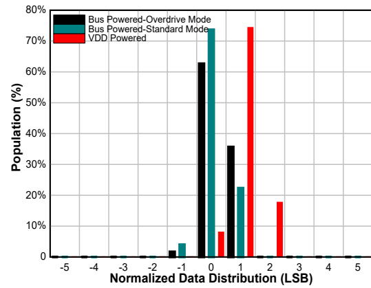
Figure 8-16. Data Distribution for Power Mode and Bus Speed
