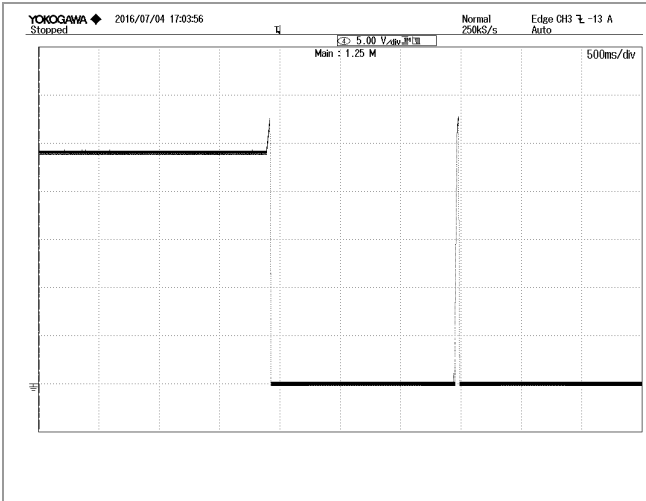
Figure 7: Output over voltage protection at 110/220Vac, 21A lout, VOUT:5V/div, 500mS/div
