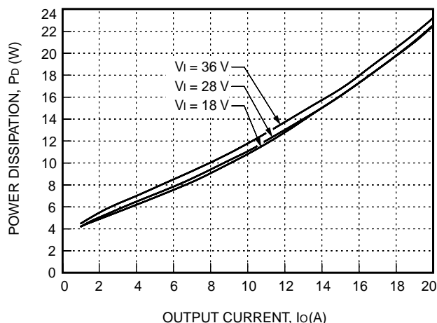
Figure 26. JC100F Power Dissipation vs. Output Current
