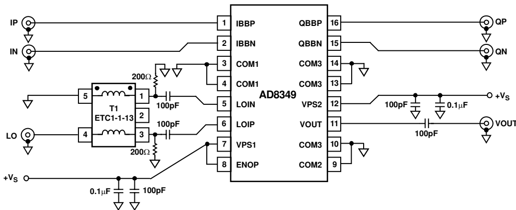
Figure 43. Basic Connections
