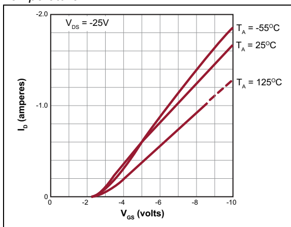
FIGURE 2-8: Transfer Characteristics.
