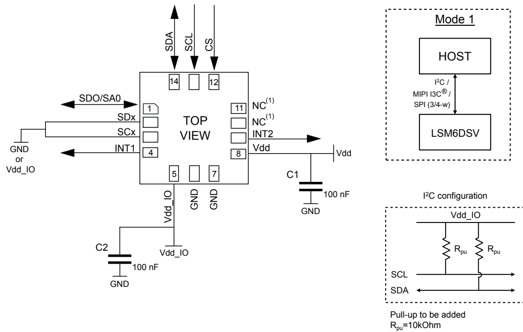
Figure 27. LSM6DSV electrical connections in mode 1
