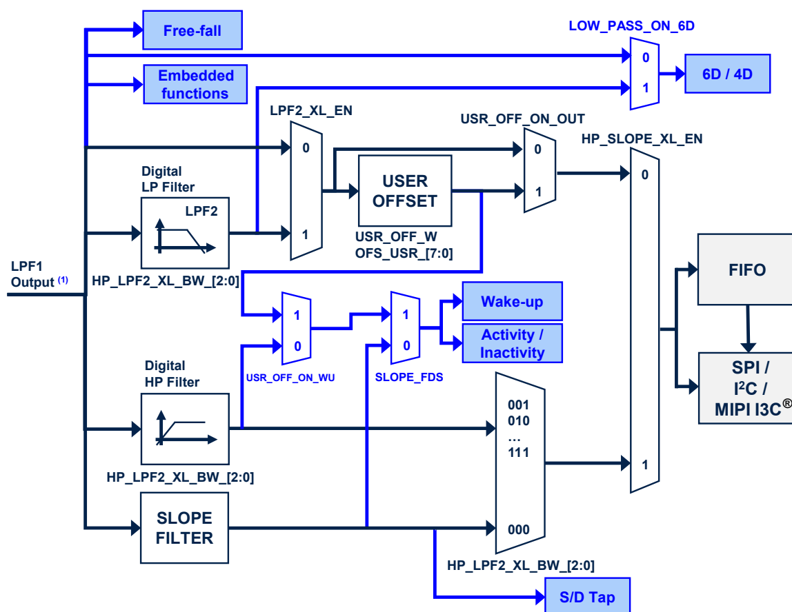
Figure 19. Accelerometer composite filter
