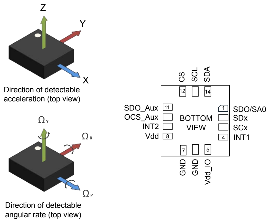
Figure 4. Pin connections
