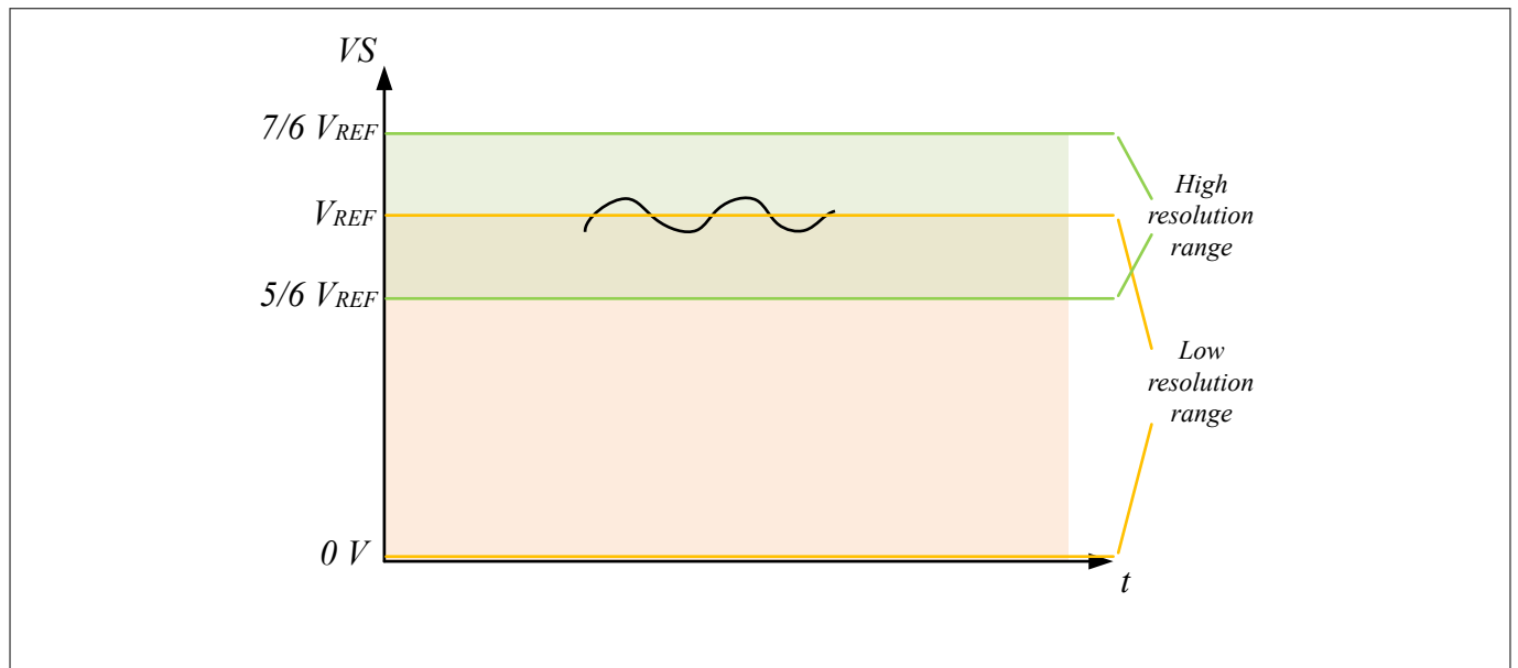
Figure 7 Sensing Ranges
