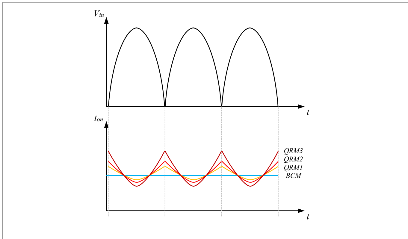
Figure 11 THD optimization on-time
