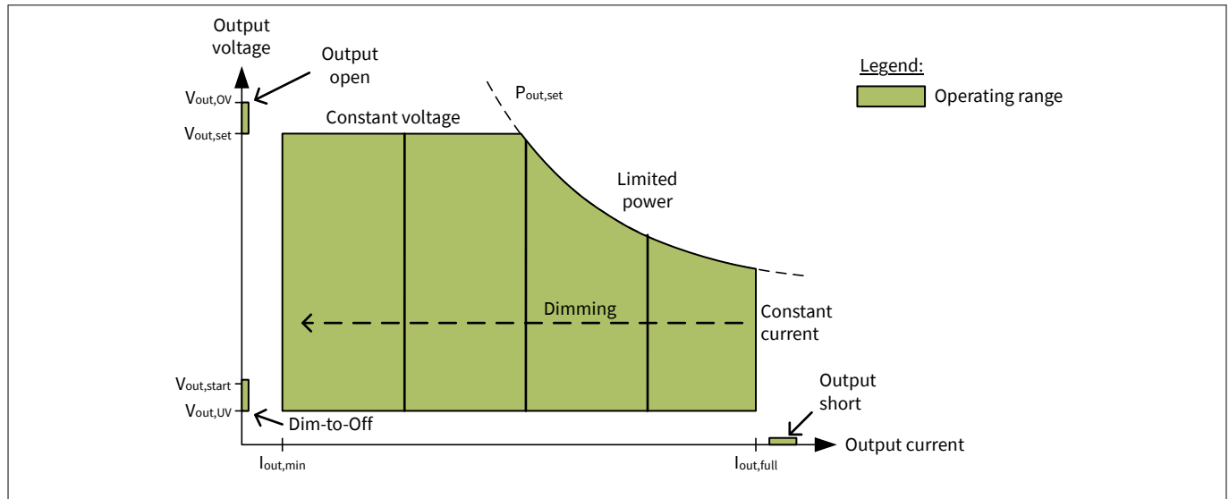
Figure 19 Control scheme for CC/CV/LP modes (including dimming)
