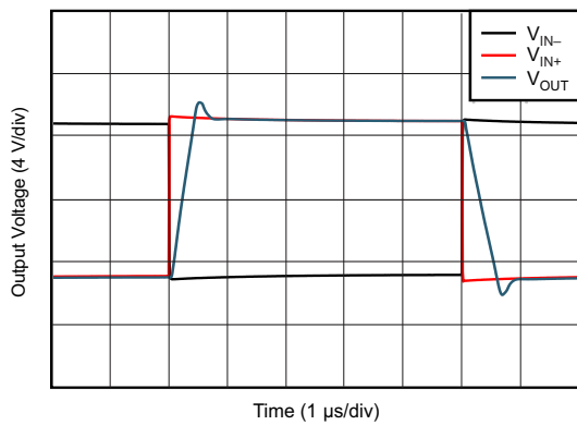
Figure 7-43. Settling Time
