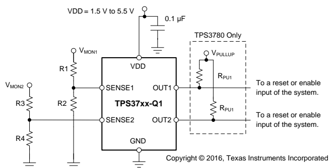
Typical Schematic
