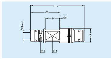
FZG Straight plug with positioning pin, cable clamp, and smooth handling surface
