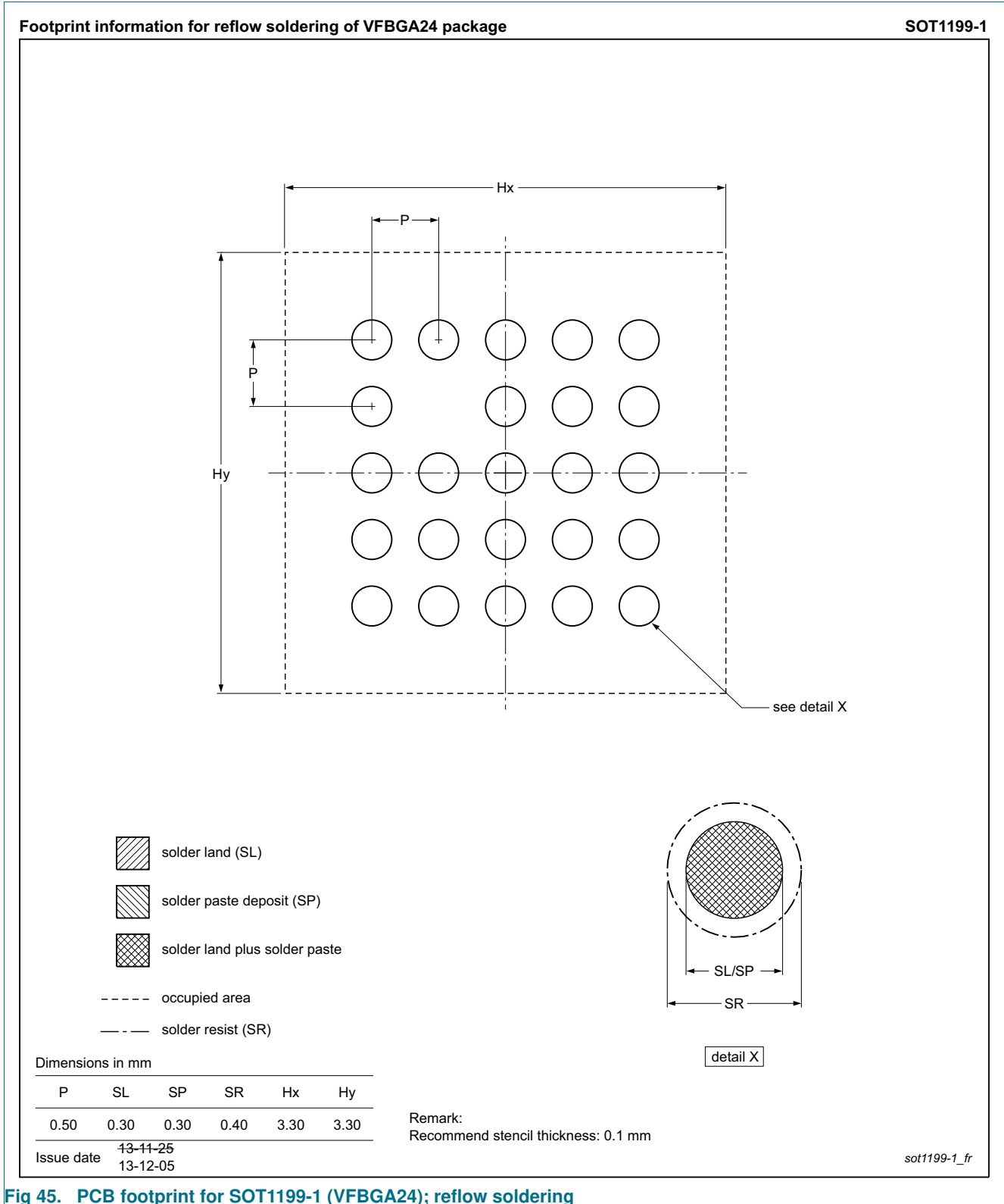
Fig 45. PCB footprint for SOT1199-1 (VFBGA24); reflow soldering
