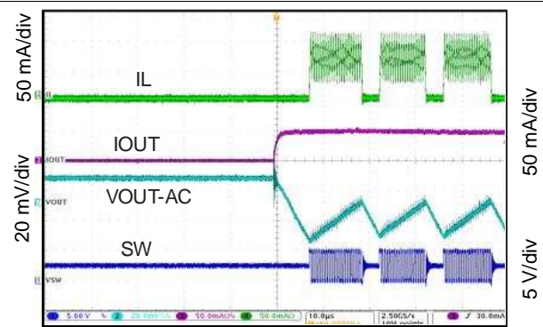
Figure 66. Sampling Waveform
