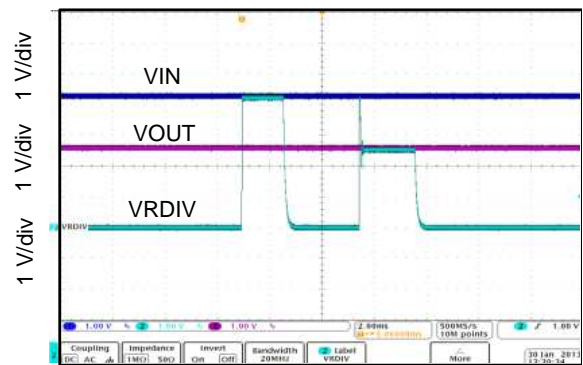
Figure 64. Steady State Operation
