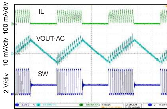
Figure 63. Steady State Operation
