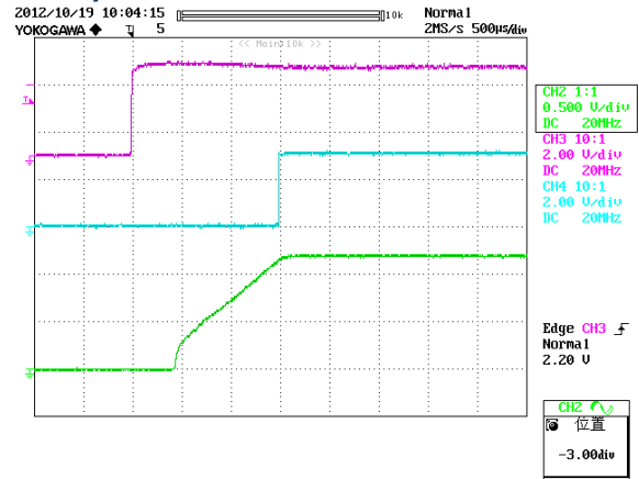
Figure 14: Turn on delay time at 12Vin, 1.2V/60A out (500µs/div)
