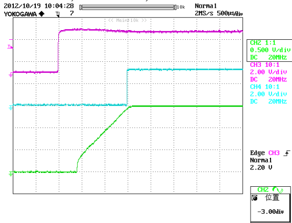
Figure 15: Turn on delay time at 12Vin, 1.5V/60A out (500µs/div)
