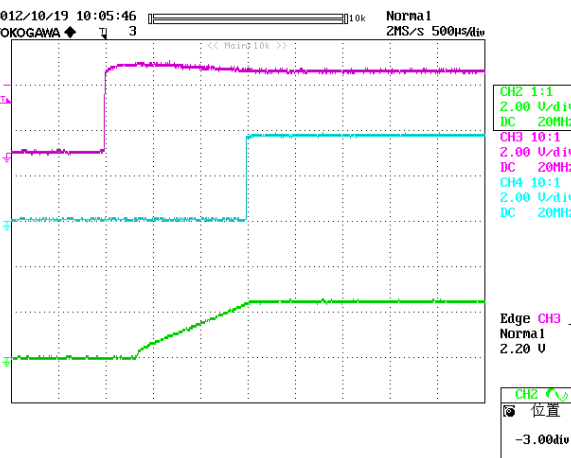
Figure 17: Turn on delay time at 12Vin, 2.5V/60A out (500µs/div)
