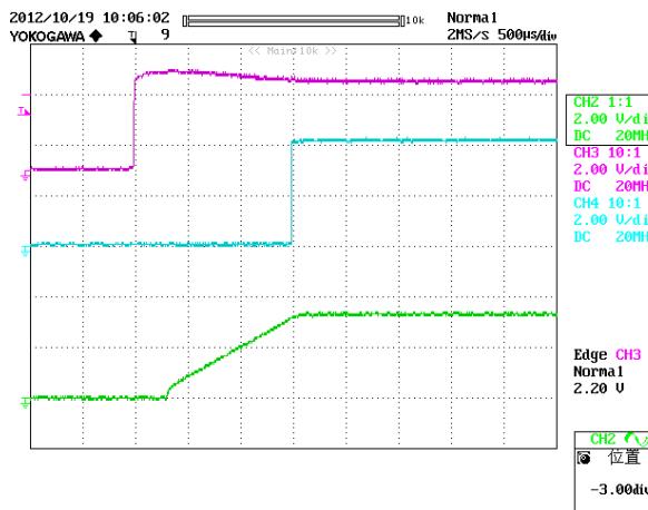
Figure 18: Turn on delay time at 12Vin, 3.3V/60A out (500µs/div)
