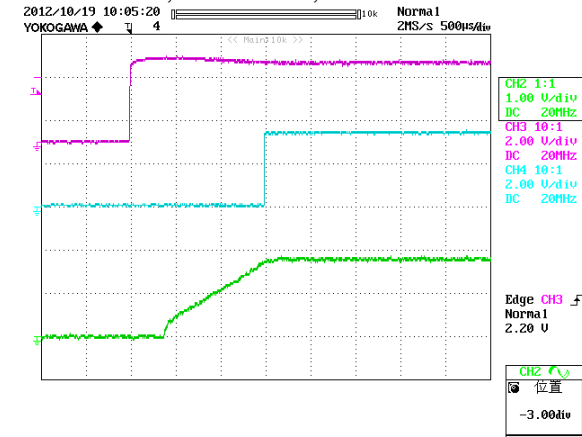
Figure 16: Turn on delay time at 12Vin, 1.8V/60A out (500µs/div)
