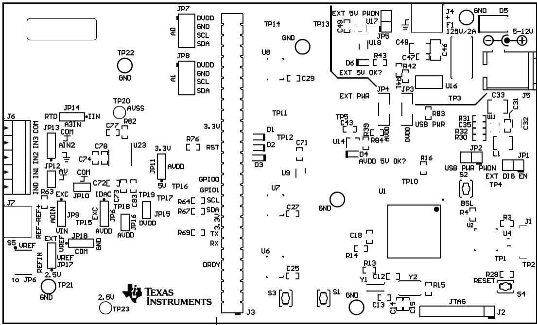
Figure 23. Top Silkscreen
