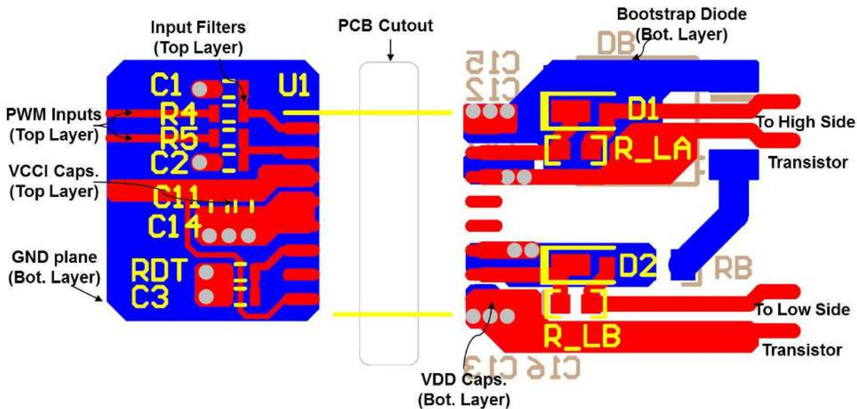
Figure 44. Layout Example
