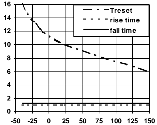
Figure 18 - Rise Time, Fall Time and Treset (ns) Vs Tj (°C)
