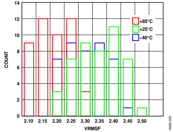
Figure 24. Distribution of VRMSF, P_{IN} = 20 \text{ dBm} , 6 GHz
