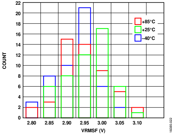
Figure 21. Distribution of VRMSF, P_{IN} = 20 \text{ dBm} , 1 GHz
