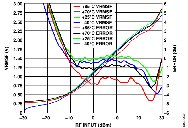
Figure 19. VRMSF and Error vs. RF Input Level and Temperature at 6 GHz, Error Calculated Using Linear Regression of Data Between 20 dBm and -5 dBm, TADJS = 0 V, TADJI = 0.2 V, CHPF+/CHPF- Open
