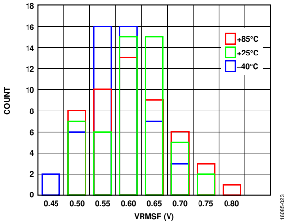
Figure 22. Distribution of VRMSF, P_{IN} = -20 \text{ dBm} , 1 GHz
