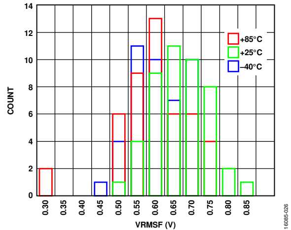
Figure 25. Distribution of VRMSF, P_{IN} = -10 \text{ dBm} , 6 GHz
