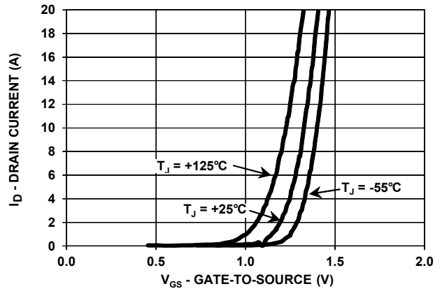
FIGURE 4. TRANSFER CHARACTERISTICS
