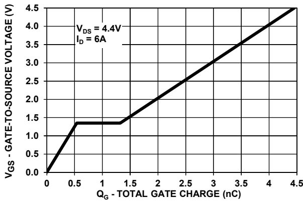
FIGURE 11. GATE CHARGE
