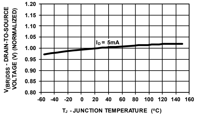
FIGURE 10. DRAIN-TO-SOURCE BREAKDOWN VOLTAGE vs JUNCTION TEMPERATURE
