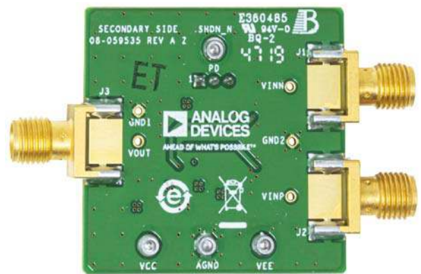
Figure 2. EVAL-LTC6228IS8, Secondary Side
