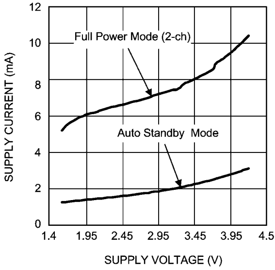
Supply Current vs Supply Voltage R_L = 16\Omega
