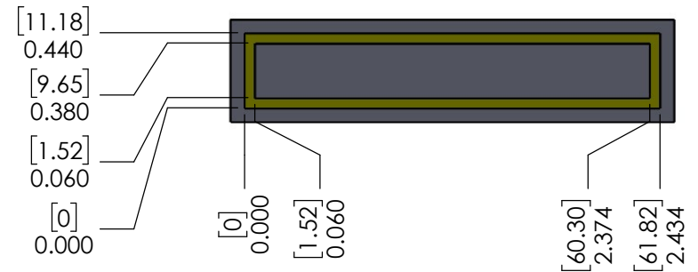
TRACE PATTERN SCALE 1:1
