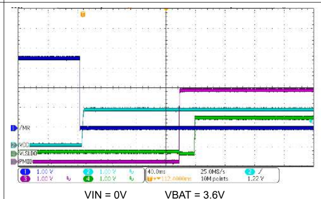
Figure 10-5. Power Up from Ship Mode with \overline{MR} Press
