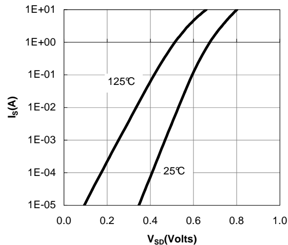
Figure 6: Body-Diode Characteristics
