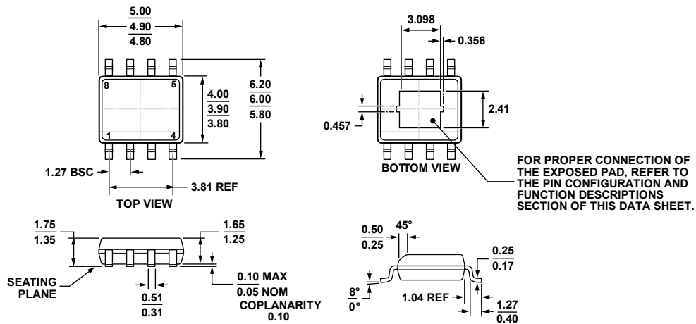
Figure 26. 8-Lead Standard Small Outline Package with Exposed Pad [SOIC_N_EP] Narrow Body (RD-8-2) Dimensions shown in millimeters
