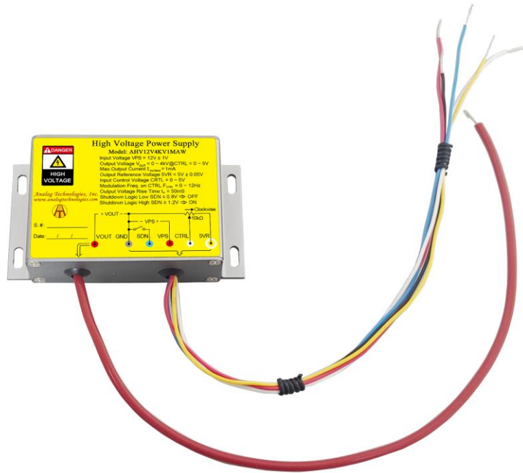
Figure 1.1. Top View of AHV12V4KV1MAW
