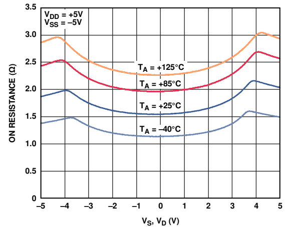
Figure 9. On Resistance as a Function of V_D ( V_S ) for Different Temperatures, \pm 5 V Dual Supply
