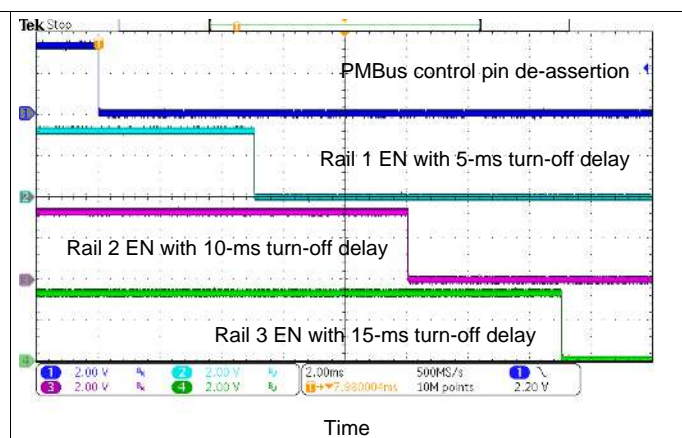
Figure 42. Shut-Down Waveforms
