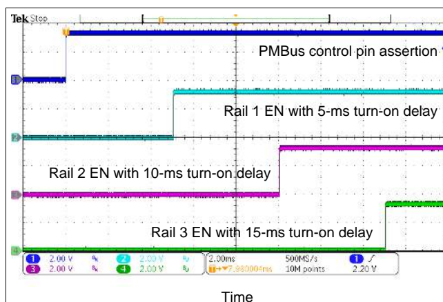
Figure 41. Start-Up Waveforms
