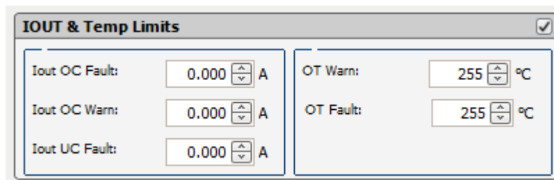
Figure 10. Current and Temperature Limits Configuration Window (Rail Config ► IOU and Temperature Limits)
