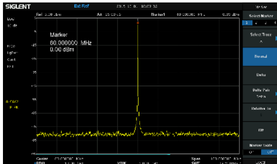
◀ High fidelity sine output. Almost no spurious observed @60MHz, 0dBm.
