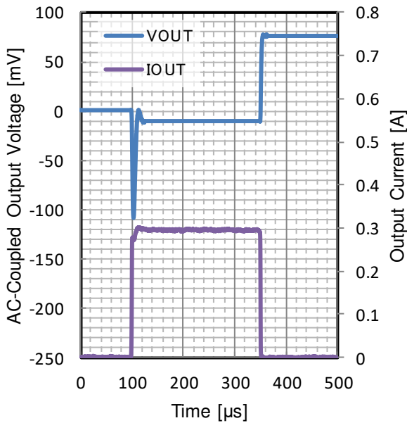
Figure 15. Load Transient
