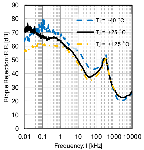
Figure 134. PSRR vs Frequency and Temperature C_{IN} = 0\ \mu\text{F} , C_{OUT} = 10\ \mu\text{F} V_{IN} = 5\text{ V} , V_{OUT} = 2.5\text{ V} , I_{OUT} = 300\text{ mA}
