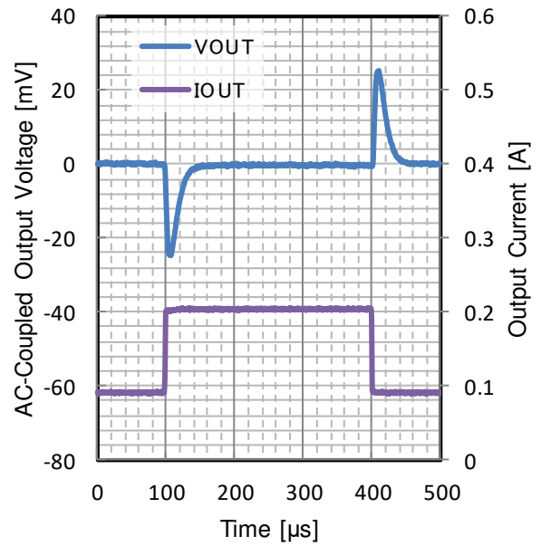
Figure 188. Load Transient
