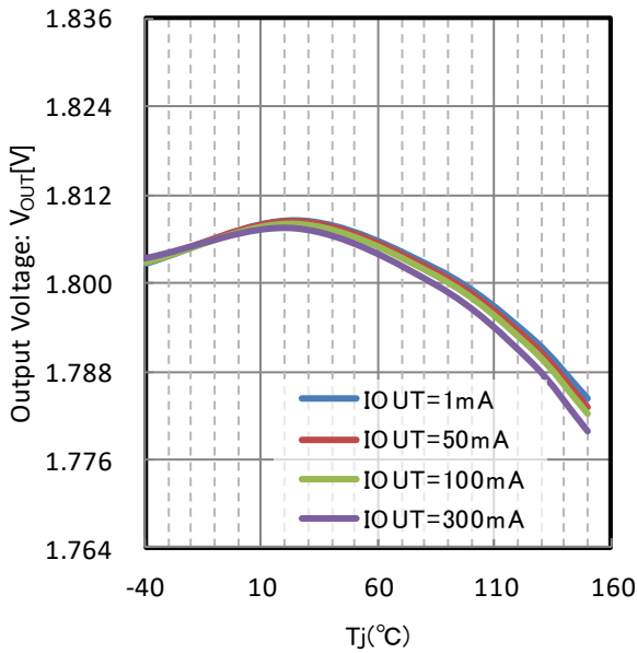
Figure 93. Output Voltage vs Junction temperature V_{OUT} = 1.8\text{ V}
