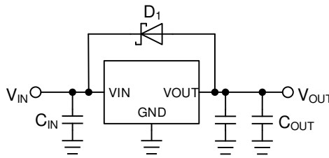
Figure 265. Bypass Diode for Reverse Current Diversion
