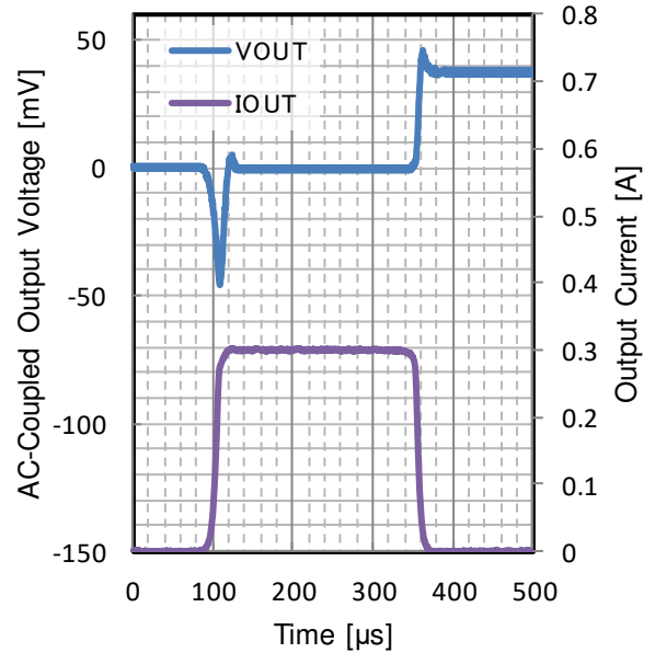
Figure 20. Load Transient
