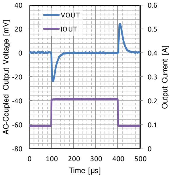
Figure 187. Load Transient
