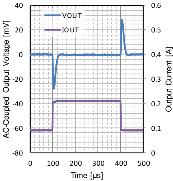
Figure 100. Load Transient
