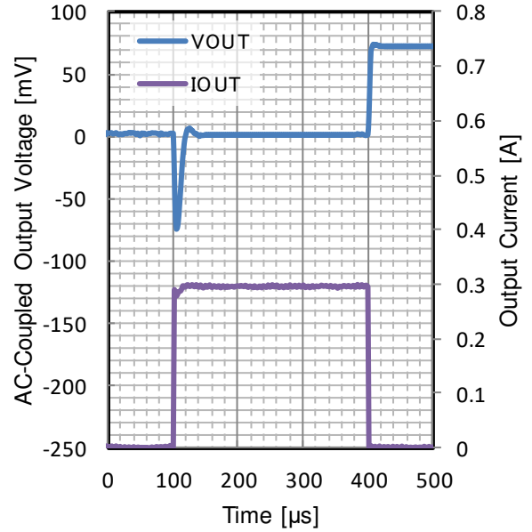
Figure 56. Load Transient
