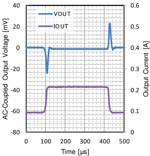
Figure 66. Load Transient
