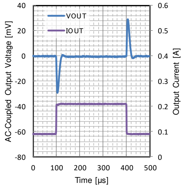
Figure 101. Load Transient
