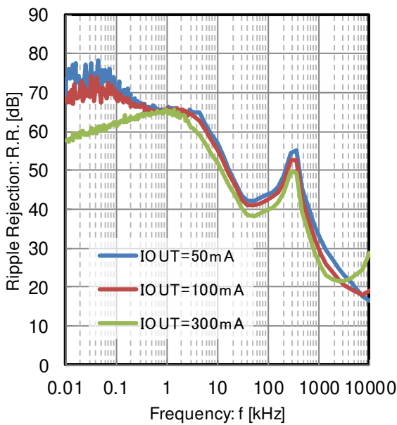
Figure 133. PSRR vs Frequency and Output Current C_{IN} = 0\ \mu\text{F} , C_{OUT} = 10\ \mu\text{F} V_{OUT} = 2.5\text{ V}
