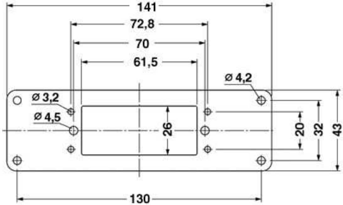
Dimensioned drawing
