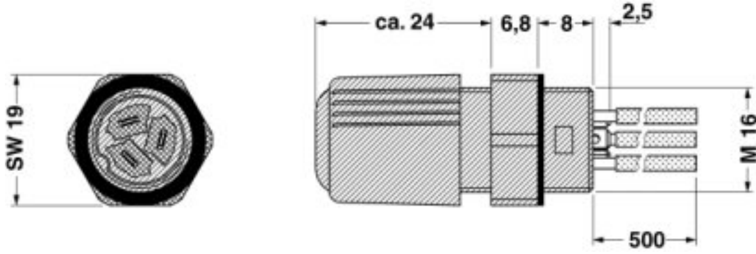
Dimensioned drawing
