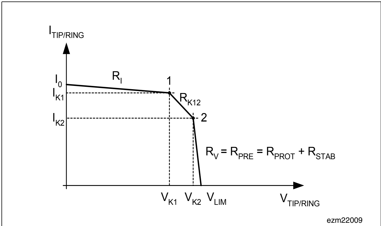
Figure 15 DC Characteristics
