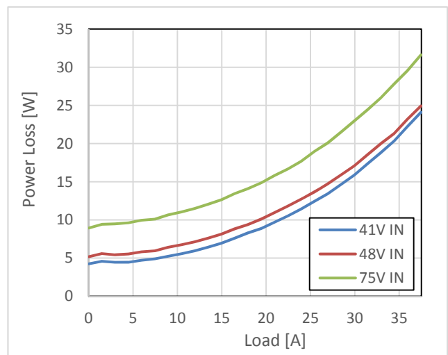
Fig.3: Power Loss vs. load current and input voltage for power module mounted horizontally with airflow 400LFM (2.0m/s) and T_a=25^{\circ}C .
