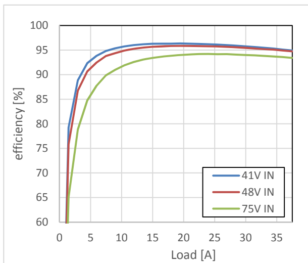
Fig.2: Efficiency vs. load current and input voltage for power module mounted horizontally with airflow 400LFM (2.0m/s) and T_a=25^{\circ}C .
