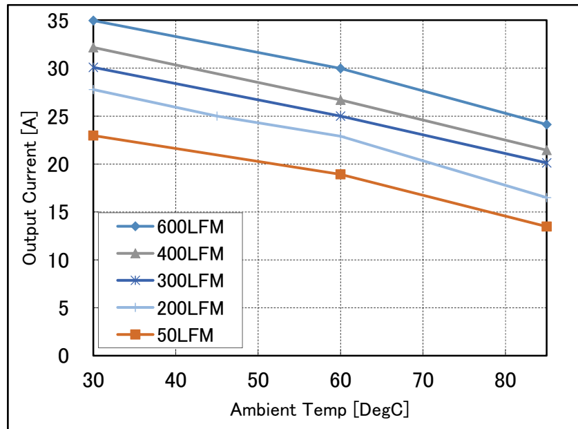
Fig.1-b: Available load current vs. ambient temperature and airflow rates for V_{in}=48V without baseplate (open frame). Airflow is from Pin 3 to Pin 1. Maximum component temperature \leq 125^{\circ}C
